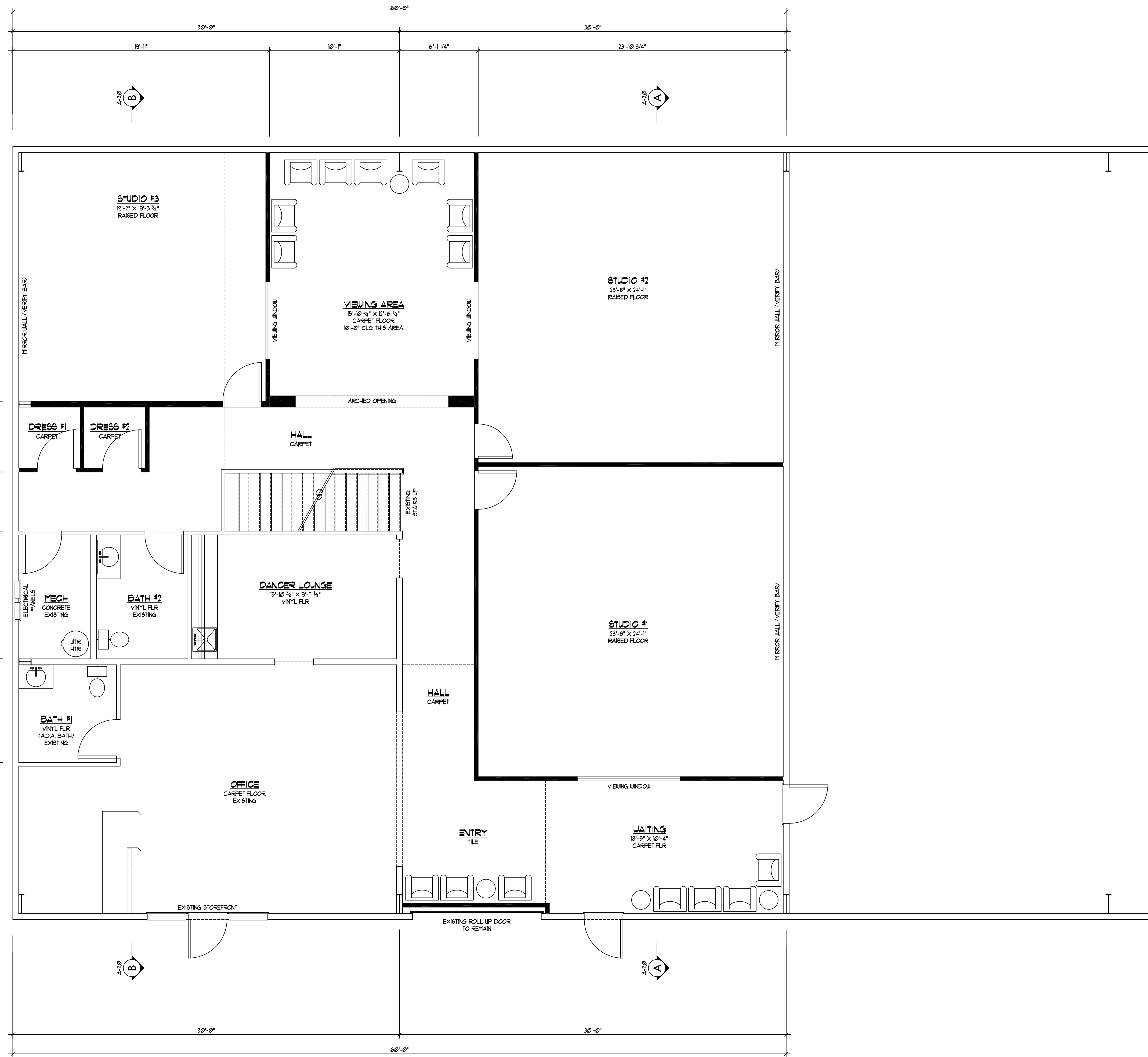
MAIN FLOOR PLAN OPTION 'A' 1/4" = 1'-0"
